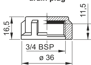
3/4" BSP female drain plug
