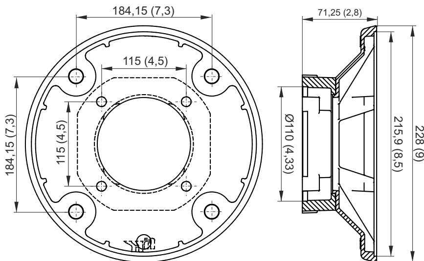
Adaptor flange
