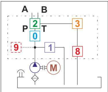
Hydraulic scheme
