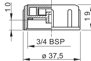
Filler breather 3/4" BSP female
