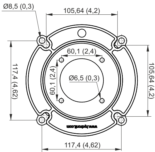
Adaptor flange
